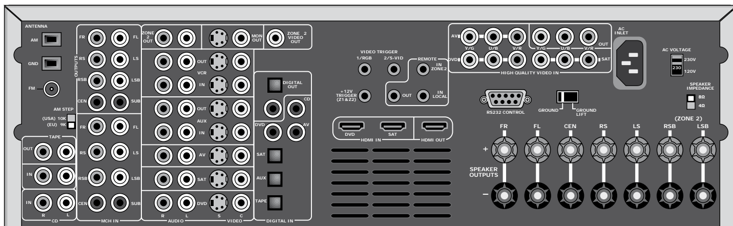
The AVR350 rear panel
